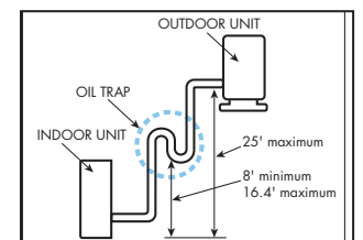
Figure A. Example: 25 ft. maximum elevation.
